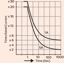
A input overload withstanding
