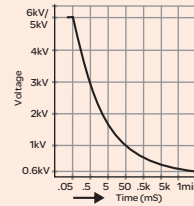
V input overload withstanding
