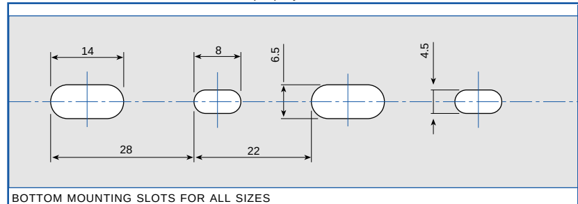
BOTTOM MOUNTING SLOTS FOR ALL SIZES
